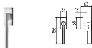
1462/DK MARTELLINA DK drehkipp system
